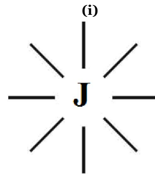
(J-Logic)
